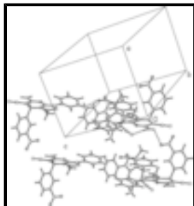
Fig. 2. Crystal packing of the title compound, viewed along the a axis. Intermolecular hydrogen bonds are shown as dashed lines.
